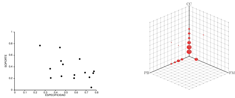
(b) SUBDUE
