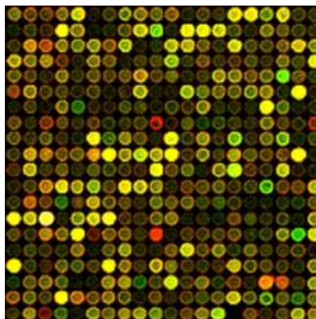
Figura 1.8: Microarray
