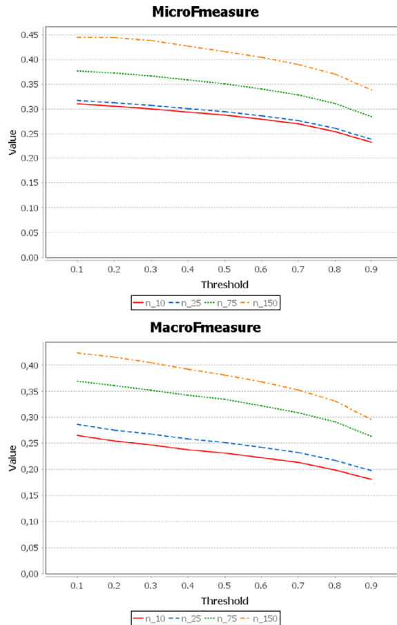
Fig. 5. Micro and macro F measures for pul-km using different thresholds, for a minimum of 10, 25, 75 and 150 interventions.
