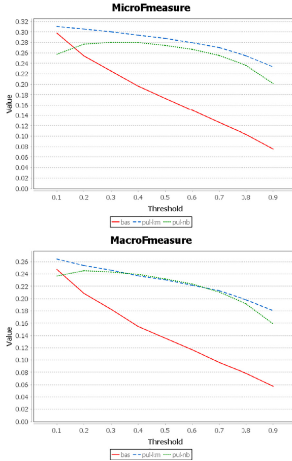
Fig. 3. Micro and macro F measures for bas , pul-km and pul-nb using different thresholds.
