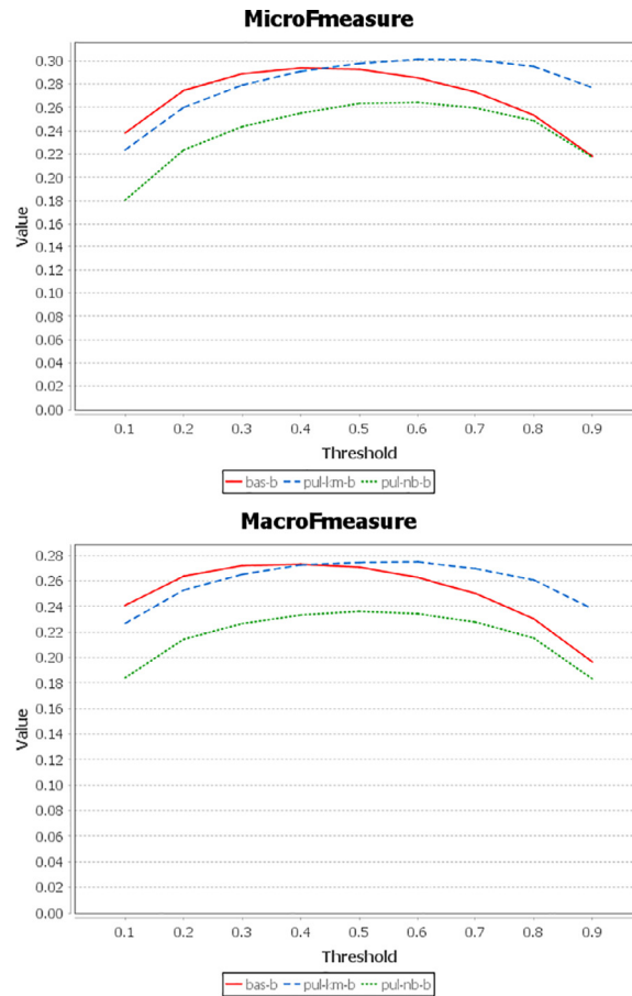
Fig. 4. Micro and macro F measures for bas-b , pul-km-b and pul-nb-b using different thresholds.
