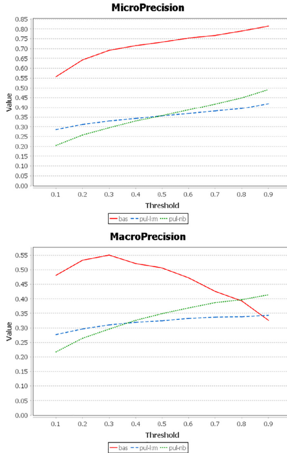
Fig. 1. Micro and macro precision for bas , pul-km and pul-nb using different thresholds.
