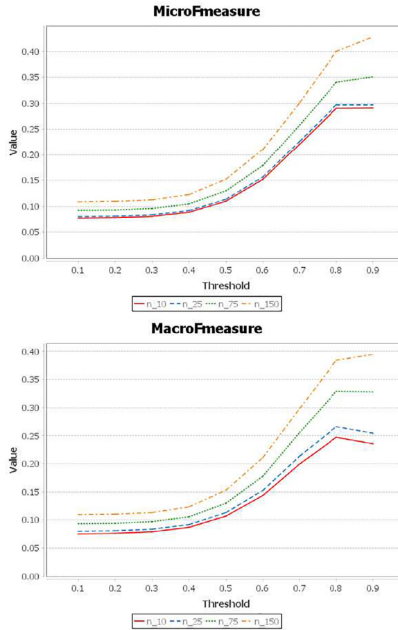
Fig. 6. Micro and macro F measures for ir-i using different thresholds, for a minimum of 10, 25, 75 and 150 interventions.
