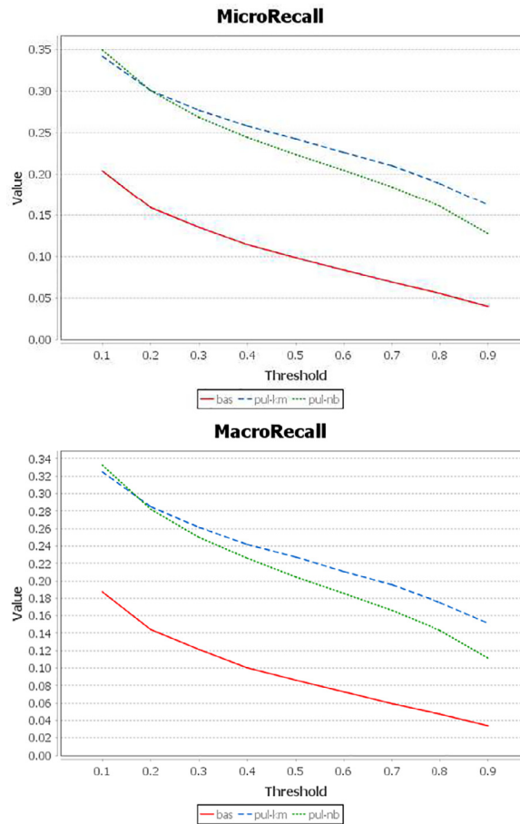
Fig. 2. Micro and macro recall for bas , pul-km and pul-nb using different thresholds.
