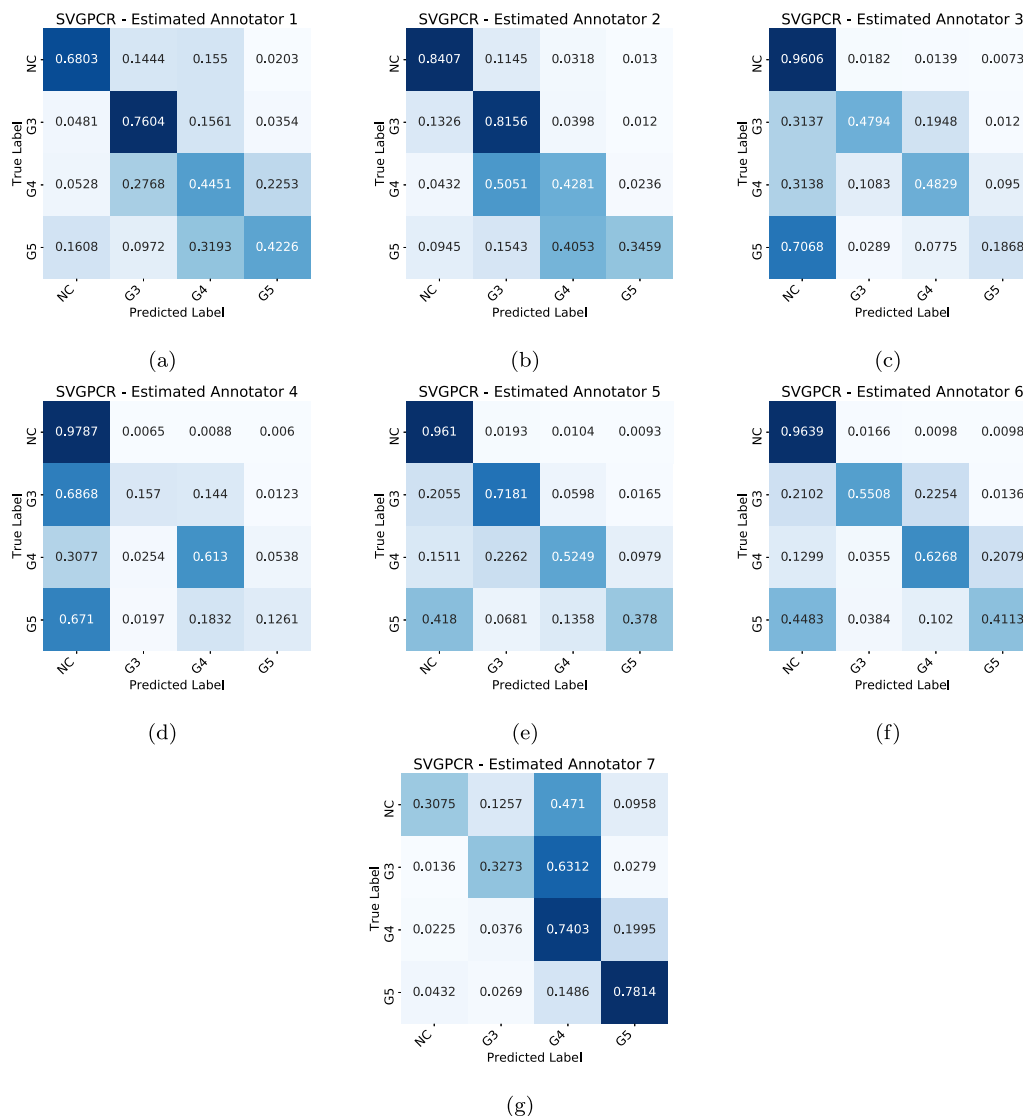
Fig. 8. Estimated confusion matrices for the seven annotators by the SVGPCR model.
