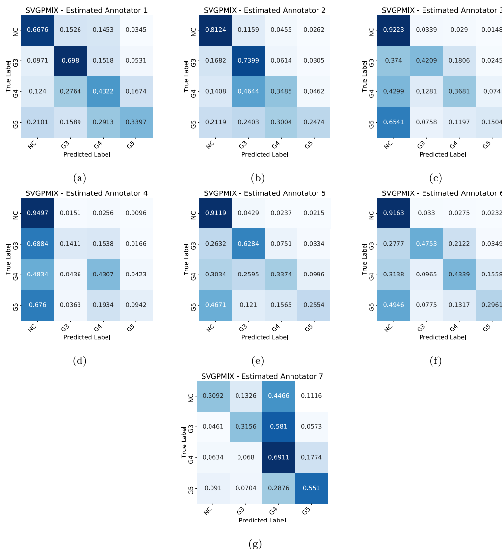
Fig. 9. Estimated confusion matrices for the seven annotators by the SVGPMIX model.
