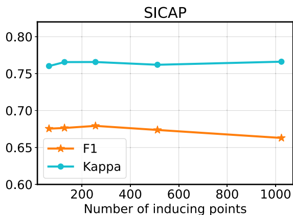
Fig. 3. Variation of the F1 and Kappa scores with the number of inducing points for the SVGP model trained on the SICAPv2 dataset. These results are reported on the validation set.
