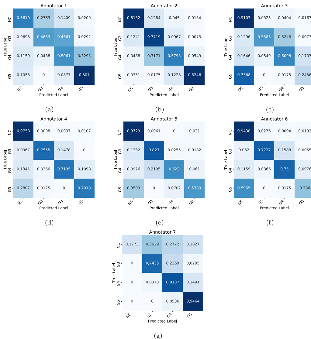
Fig. 7. Normalized confusion matrices of the seven annotators in the CrowdGleason curated test set.
