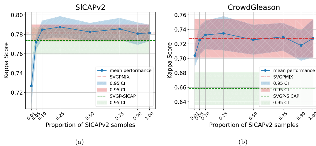
Fig. 6. Results of the SVGPMIX model varying the proportion expert-labeled samples from SICAPv2.
