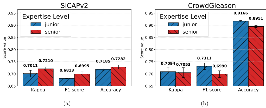
Fig. 4. Results of the SVGPCR model trained with labels provided by junior participants (first and second year) or senior participants (third and fourth year).
