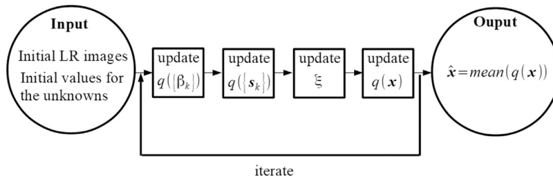
Fig. 2. Graphical description of the inference process.
